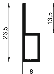
10 48 08 Rail simple 8 mm
