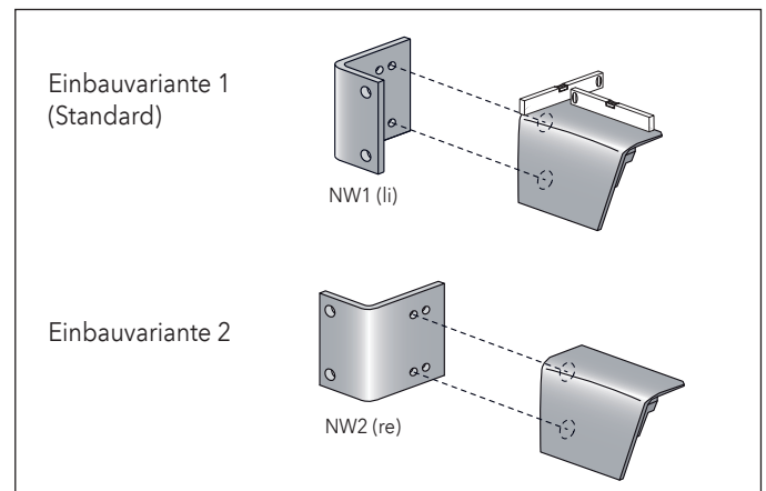
Abb. 18: Montagevariante beachten
